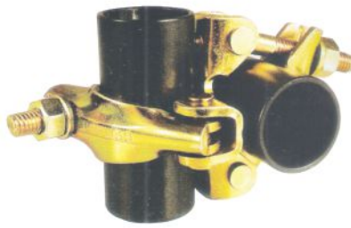
JK-02 PRESSED DOUBLE COUPLER FOR TUBE OD 48.3mm (EN-74/BS-1139)
